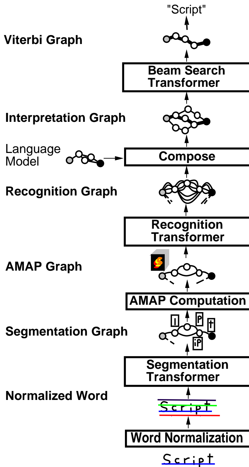
Figure 30: An on-line handwriting recognition GTN based on heuristic over-segmentation
