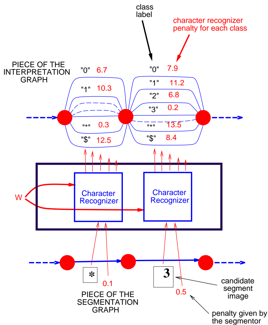
Figure 18: The recognition transformer refines each arc of the segmentation arc into a set of arcs in the interpretation graph, one per character class, with attached penalties and labels.
