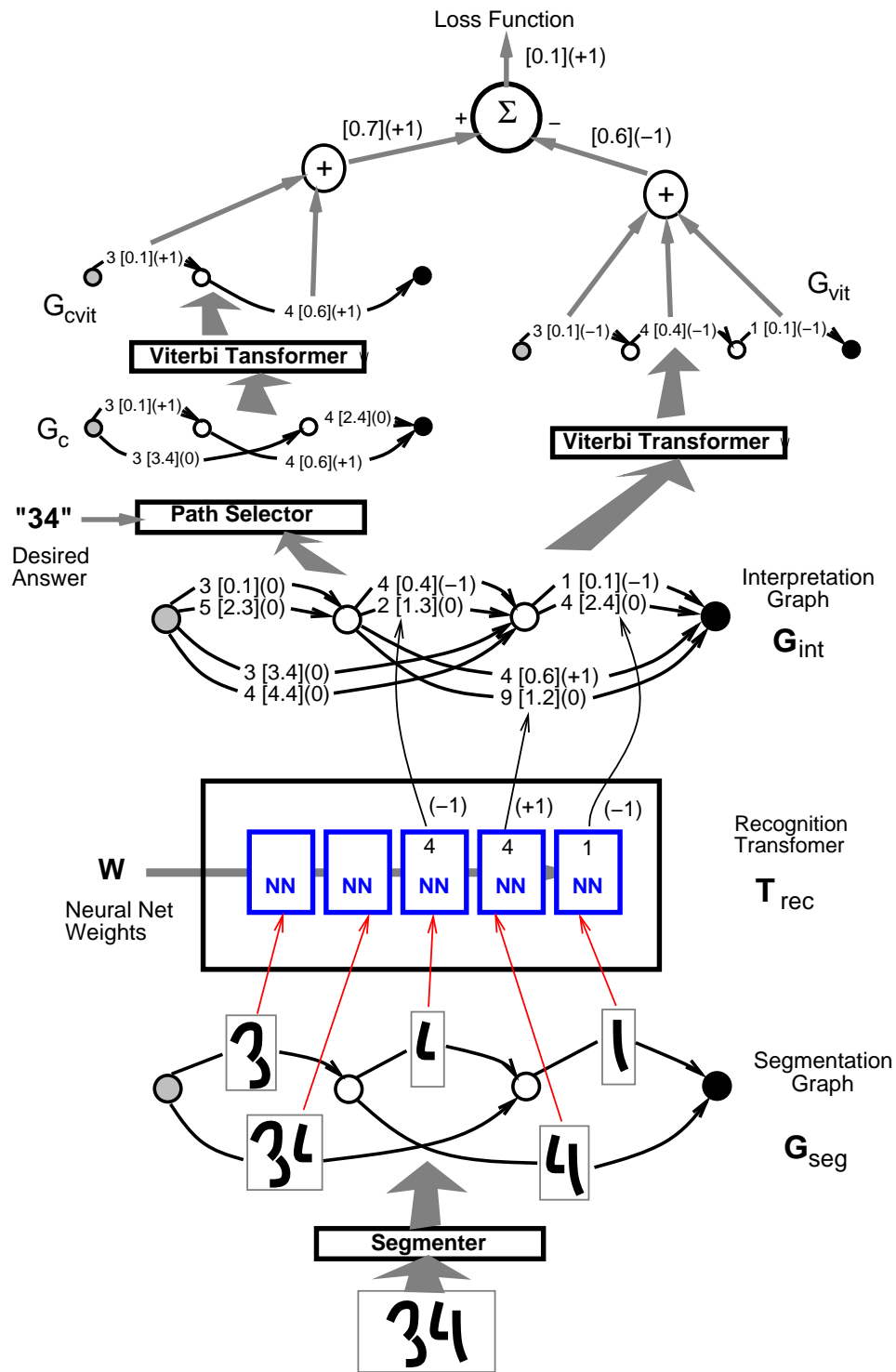
Figure 20: Discriminative Viterbi Training GTN Architecture for a character string recognizer based on Heuristic Over-Segmentation. Quantities in square brackets are penalties computed during the forward propagation. Quantities in parentheses are partial derivatives computed during the backward propagation.
