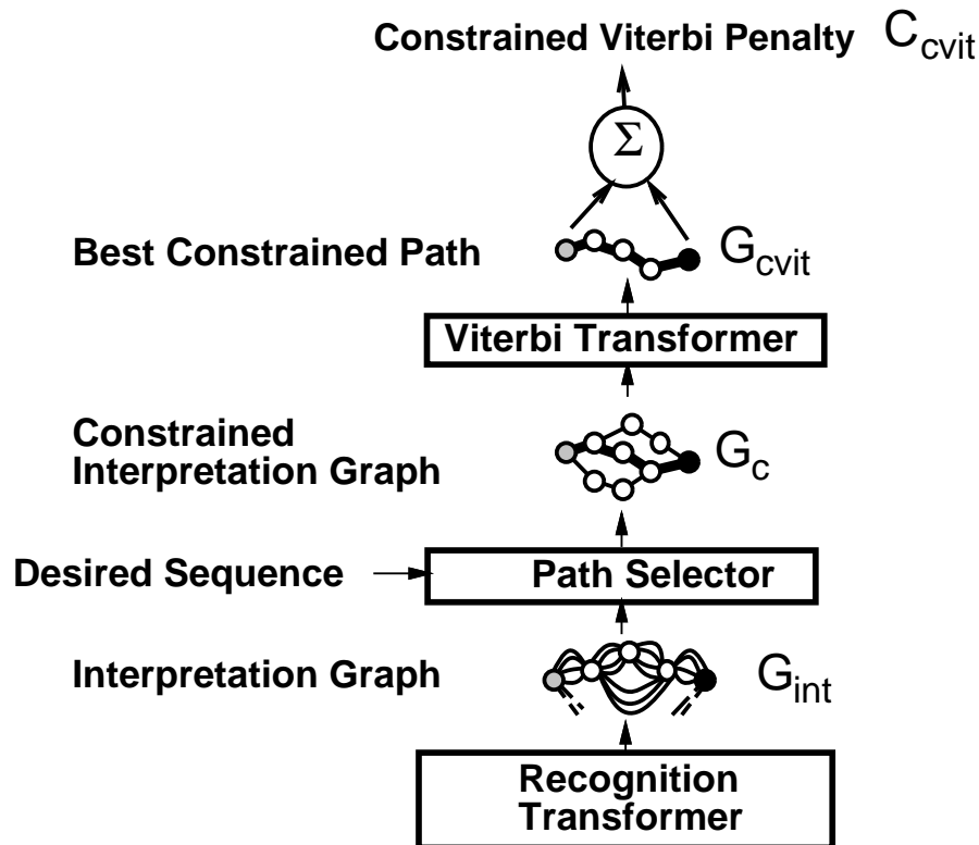
Figure 19: Viterbi Training GTN Architecture for a character string recognizer based on Heuristic Over-Segmentation.
