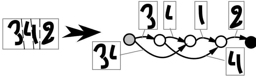
Figure 16: Building a segmentation graph with Heuristic Over-Segmentation.
