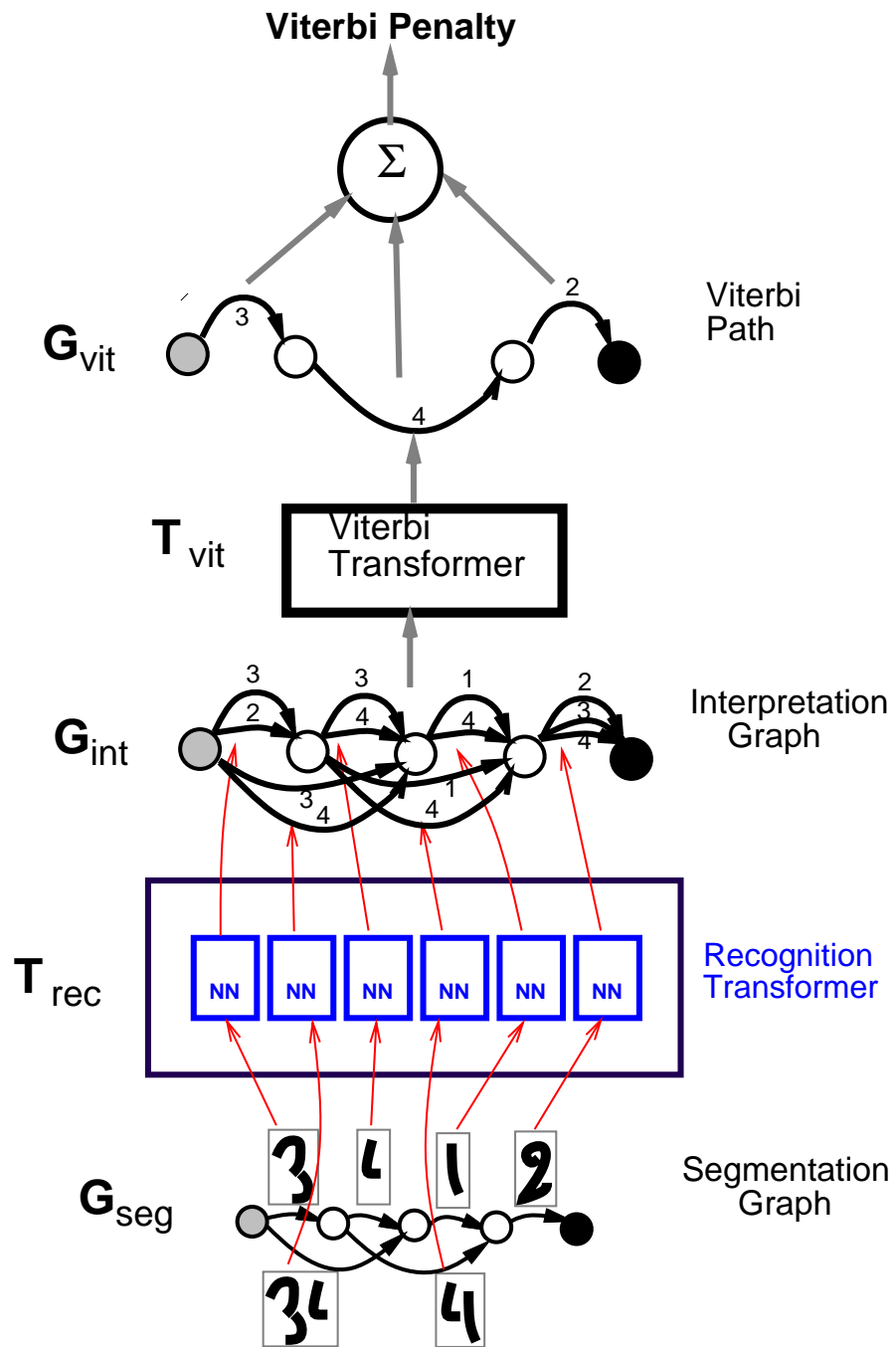
Figure 17: Recognizing a character string with a GTN. For readability, only the arcs with low penalties are shown.
