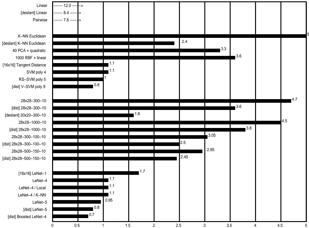
Figure 9: Error rate on the test set (%) for various classification methods. [deslant] indicates that the classifier was trained and tested on the deslanted version of the database. [dist] indicates that the training set was augmented with artificially distorted examples. [16x16] indicates that the system used the 16x16 pixel images. The uncertainty in the quoted error rates is about 0.1%.
