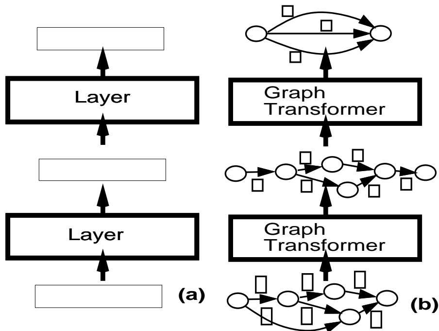
Figure 15: Traditional neural networks, and multi-module systems communicate fixed-size vectors between layer. Multi-Layer Graph Transformer Networks are composed of trainable modules that operate on and produce graphs whose arcs carry numerical information.
