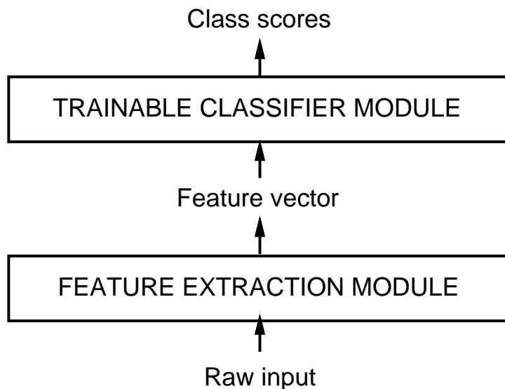
Figure 1: Traditional pattern recognition is performed with two modules: a fixed feature extractor, and a trainable classifier.
