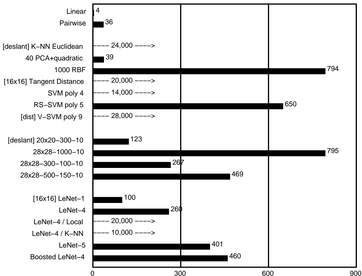
Figure 11: Number of multiply-accumulate operations for the recognition of a single character starting with a size-normalized image.
