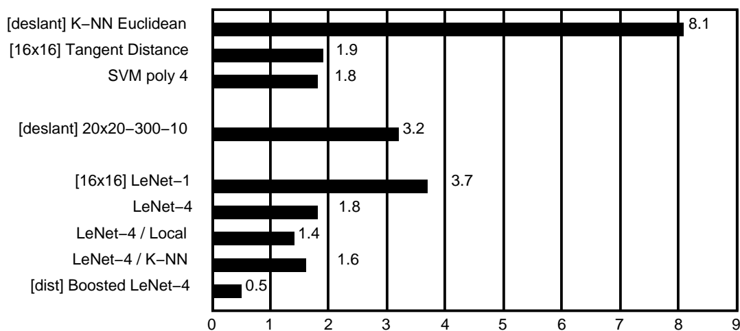
Figure 10: Rejection Performance: percentage of test patterns that must be rejected to achieve 0.5% error for some of the systems.
