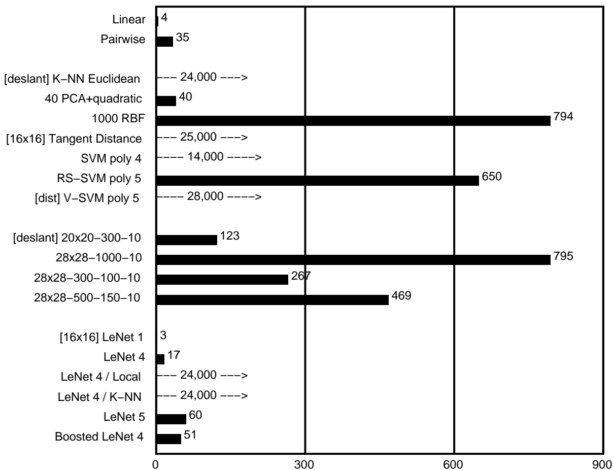
Figure 12: Memory requirements, measured in number of variables, for each of the methods. Most of the methods only require one byte per variable for adequate performance.
