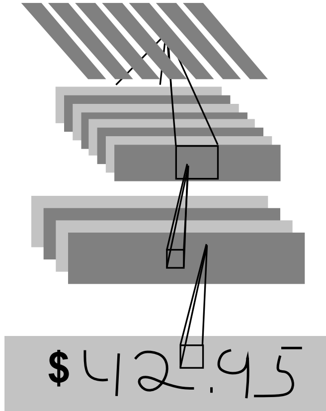
Figure 23: A Space Displacement Neural Network is a convolutional network that has been replicated over a wide input field.
