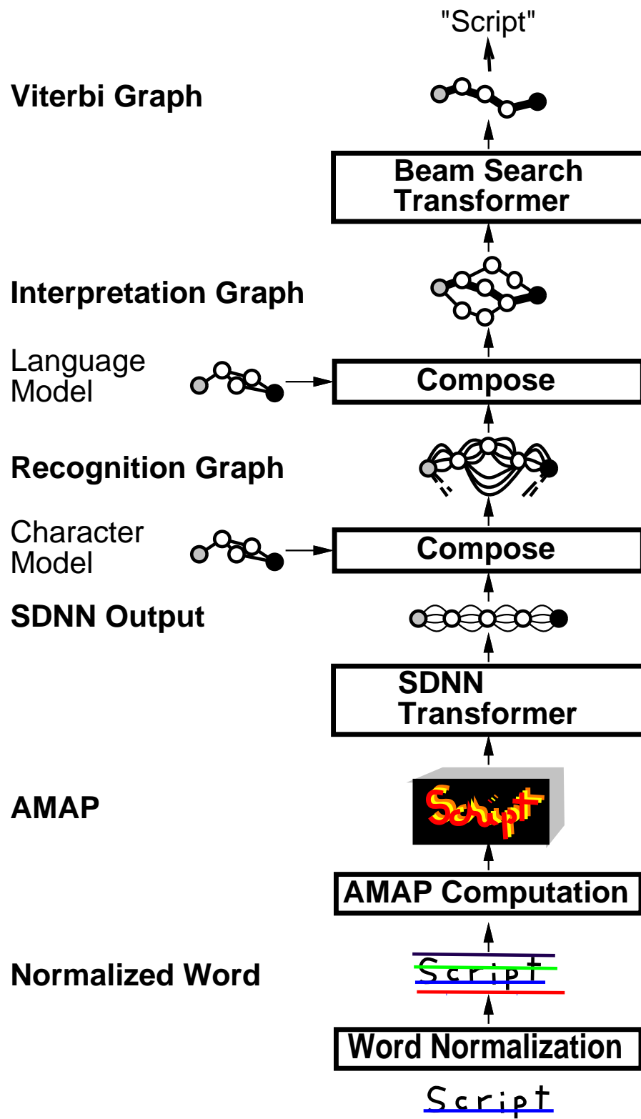
Figure 31: An on-line handwriting recognition GTN based on Space-Displacement Neural Network
